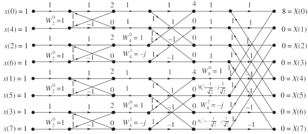
Figure 7.36 Computation of 8-point DF^\dagger of x(n) by radix-2, DI^\dagger FF^\dagger .
